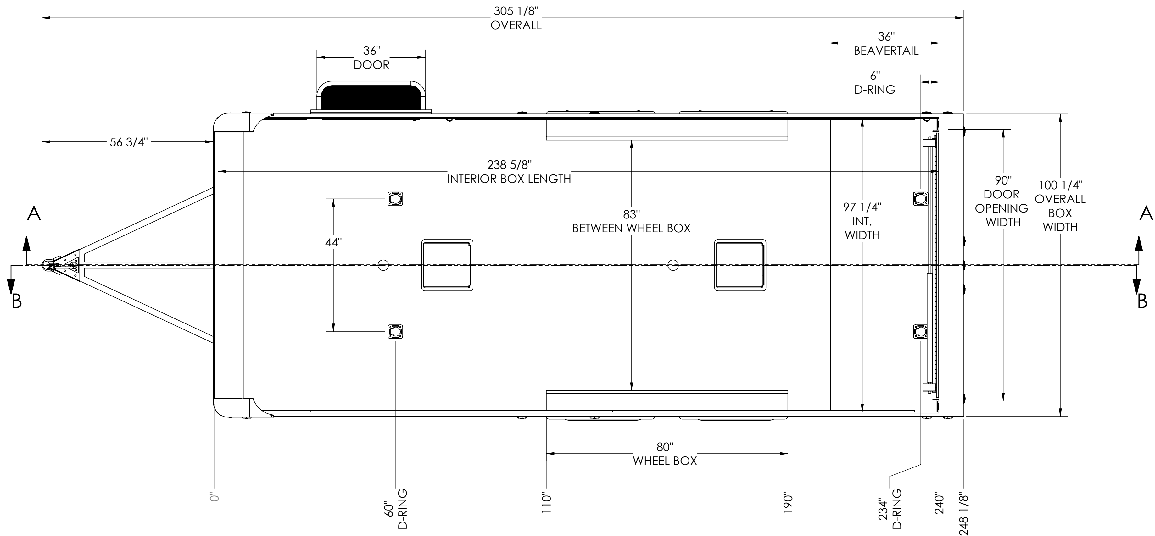
TOP VIEW STANDARD FLOOR LAYOUT
