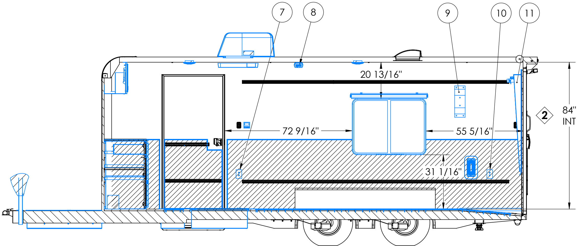
SECTION C-C
